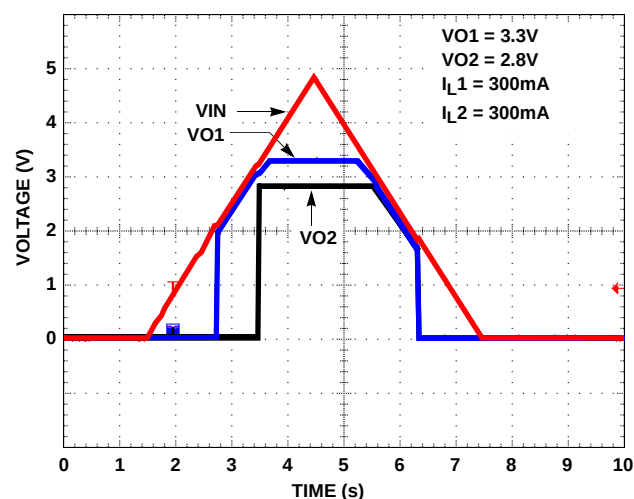
FIGURE 12. POWER-UP/POWER-DOWN
