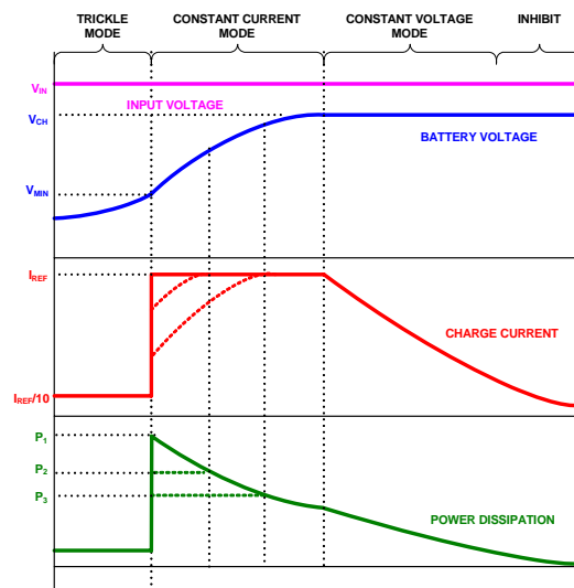
FIGURE 18. TYPICAL CHARGE CURVES USING A CONSTANT-VOLTAGE ADAPTER
