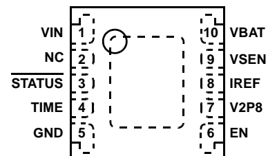
ISL9203A (10 LD 3x3 DFN) TOP VIEW
