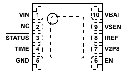
ISL9203R5220 (3x3 DFN) TOP VIEW
