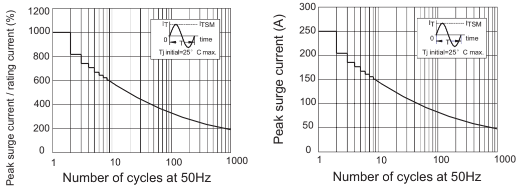
TRIAC AC switch output Maximum permissible non-repetitive peak surge current vs. Number of cycles
