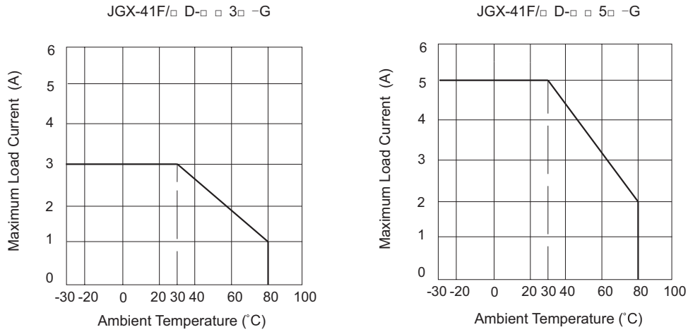
Figure 1 Maximum load current vs. ambient temperature
