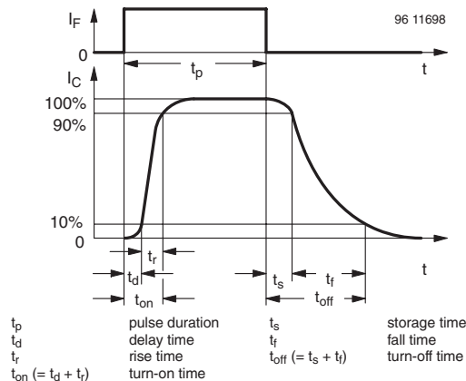
Figure 3. Switching Times
