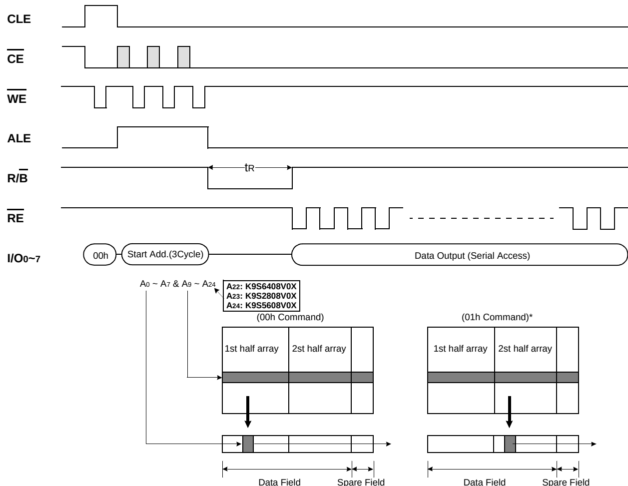
Figure 7. Read1 Operation
