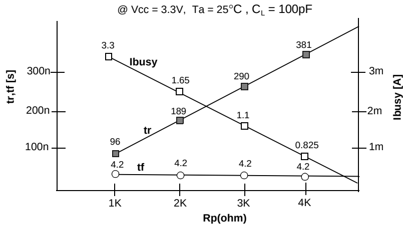
Figure 15. R_p vs t_r , t_f & R_p vs i_{busy}
