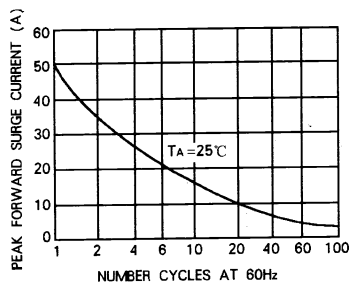
FIG. 1-MAXIMUM NON-REPETITIVE PEAK FORWARD SURGE CURRENT - PER ELEMENT
