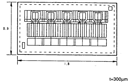
KGL2115 Prescaler
