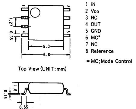
KGL2115 Prescaler
