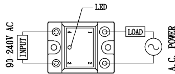
Fig.8 WIRING DIAGRAM
