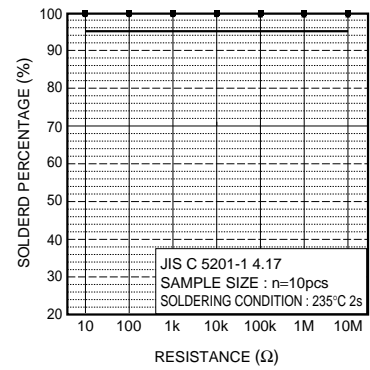
Fig.10 Solderability
