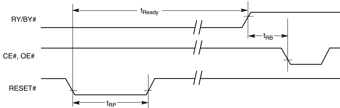
Figure 16. Reset Timings
