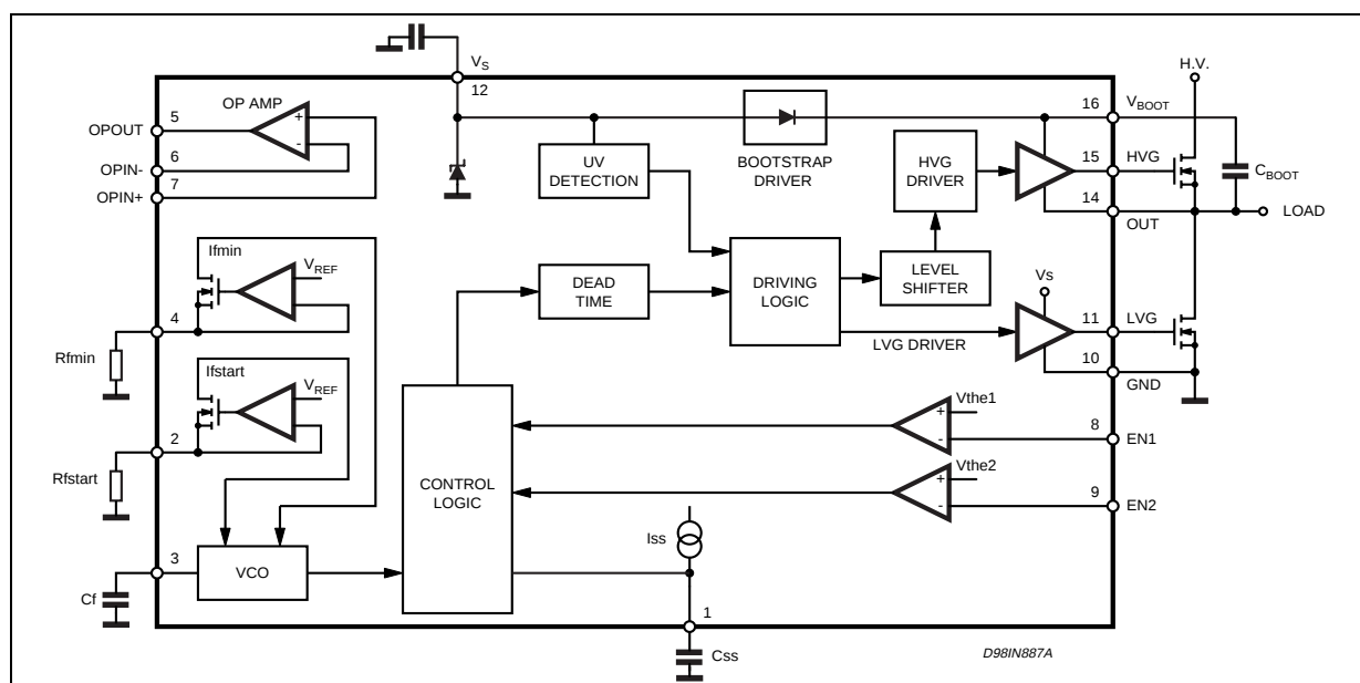
Figure 2. Block Diagram
