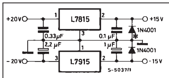
Figure 2 : Split Power Supply ( \pm 15V/1A ).
