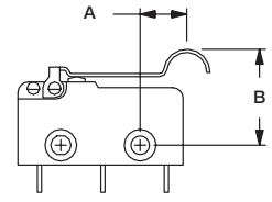
FIG. 6 Simulated Roller
