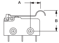
FIG. 5 Simulated Roller
