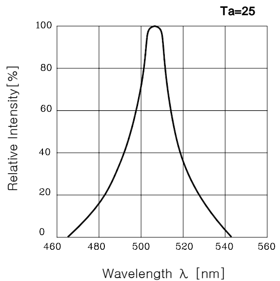
Fig. 3 Spectrum Distribution
