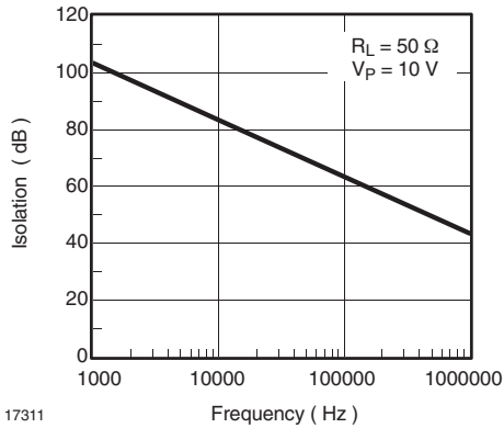
Fig. 12 Output Isolation
