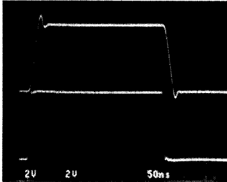
Step Response; A_V = +1
