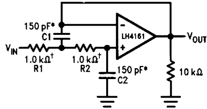
1 MHz Low-Pass Filter f_c = \frac{1}{2\pi} \sqrt{\frac{R_1 R_2 C_1 C_2}{R_1 R_2}}
