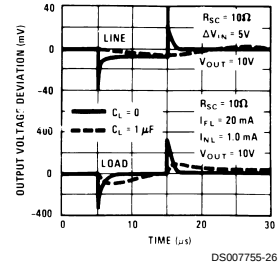
Transient Response
