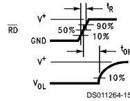
FIGURE 9. TRI-STATE Test Circuits and Waveforms
