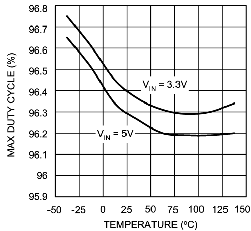
Max. Duty Cycle vs Temperature - "Y"
