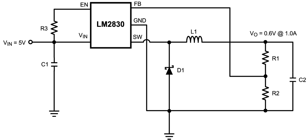
FIGURE 7. LM2830X (1.6MHz): V_{IN} = 5V , V_O = 0.6V @ 1.0A
