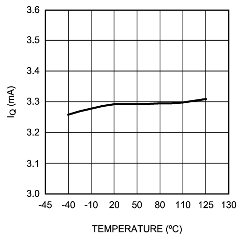
LM2830X I_Q (Quiescent Current)
