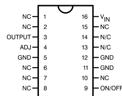
16-Lead Ceramic Surface Mount Package
