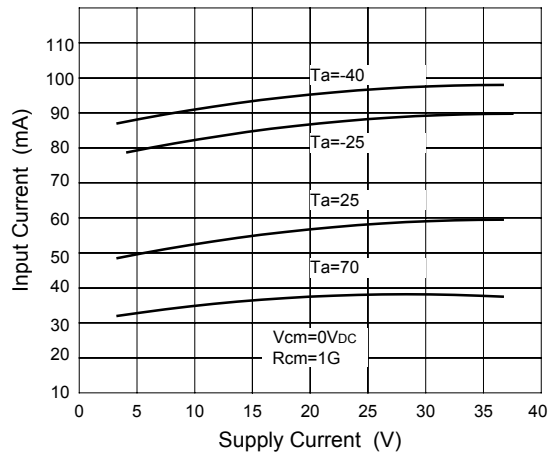
Fig.2 Input Current
