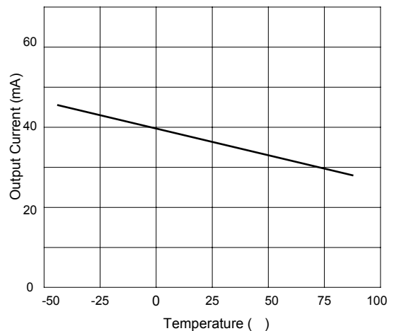
Fig.11 Current Limiting
