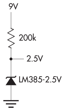
MICROPOWER REFERENCE FROM 9V BATTERY
