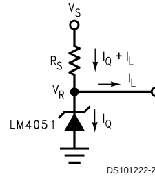
FIGURE 1. Shunt Regulator
