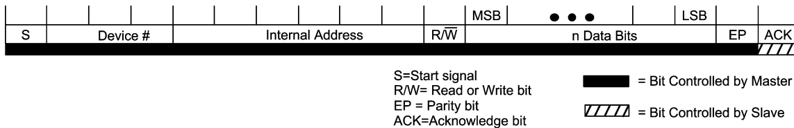
FIGURE 6. Write Transaction, master write data to LM41
