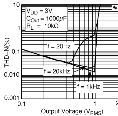
THD+N vs Output Voltage Line Out Pins
