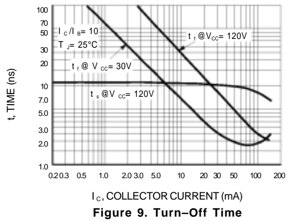
Figure 9. Turn-Off Time
