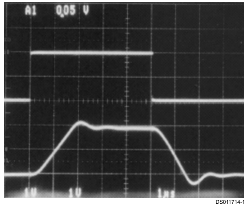
FIGURE 7. Pulse Response of LMC6484 Circuit in Figure 6
