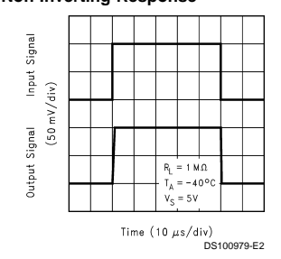
Small Signal Non-Inverting Response
