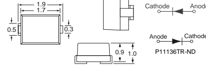
Fig. 4 — J-Lead-S Type
