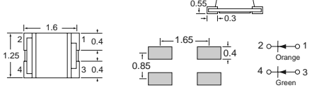
Fig. 11 — TSS Bi-Color Type
