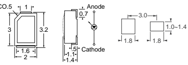
Fig. 10 — J-Lead-S Type
