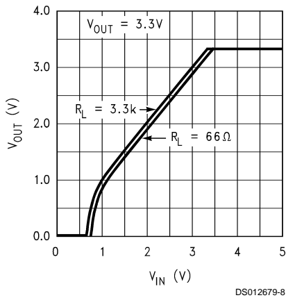
Dropout Characteristics
