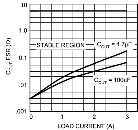
Minimum ESR vs Output Load Current
