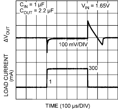
Load Transient, V_{OUT} = 1.2\text{V}
