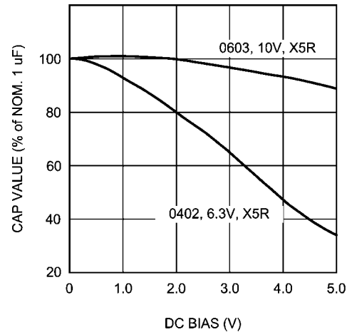
FIGURE 1. Effect of DC bias on Capacitance Value.
