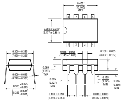
N8 Package 8-Lead PDIP (Narrow 0.300) (LTC DWG # 05-08-1510)
