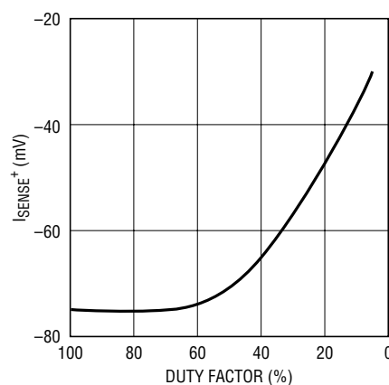
Minimum Current Sense Threshold vs Duty Factor (Buck)
