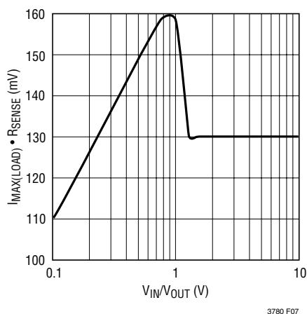
Figure 7. Load Current vs V_{IN}/V_{OUT}
