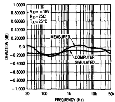
Measured Deviation from RIAA Response. Input @ 1kHz = 1mV RMS Pre-Emphasized.
