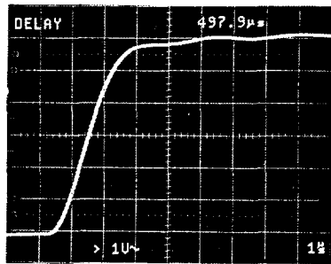
RISETIME OF PRE-AMP A_V = 20\text{dB} V_{IN} = 400\text{mV} 2kHz SQUARE WAVE MEASURED AT SINGLE ENDED OUTPUT BEFORE TRANSFORMER
