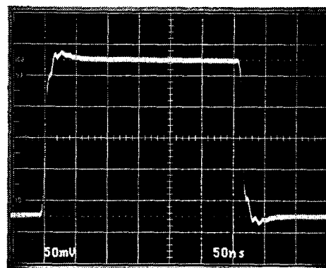
A_V = -1 , IN DEMO BOARD, C_L = 50\text{pF} WITH 10Ω ISOLATING RESISTOR
