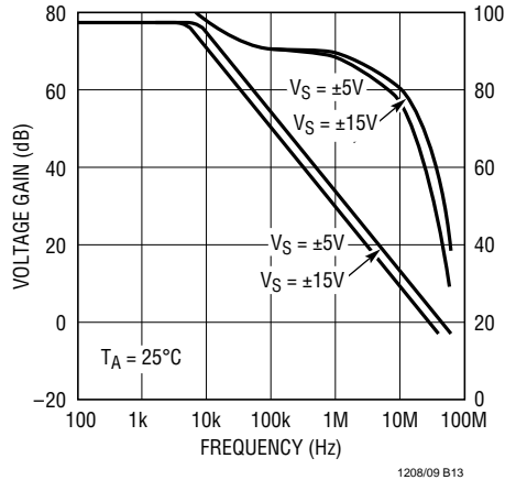
Voltage Gain and Phase vs Frequency
