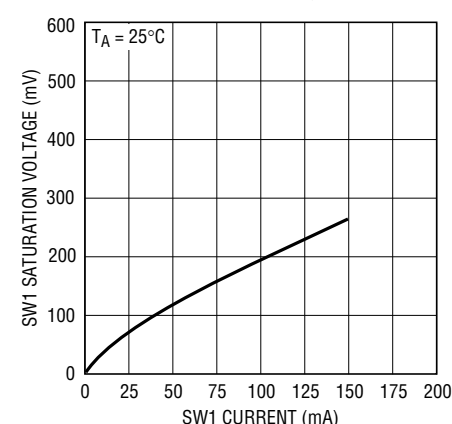
SW1 Saturation Voltage
