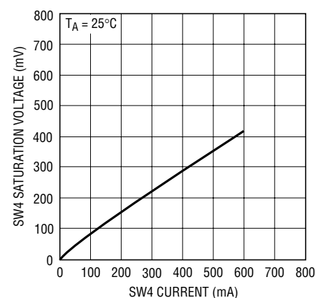
SW4 Saturation Voltage
