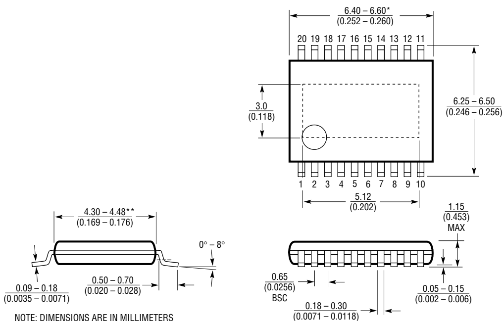
FE Package 20-Lead Plastic TSSOP (4.4mm) (LTC DWG # 05-08-1663)
