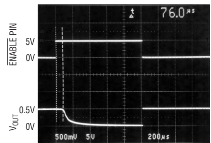
\overline{ENABLE} Pin Response Time
