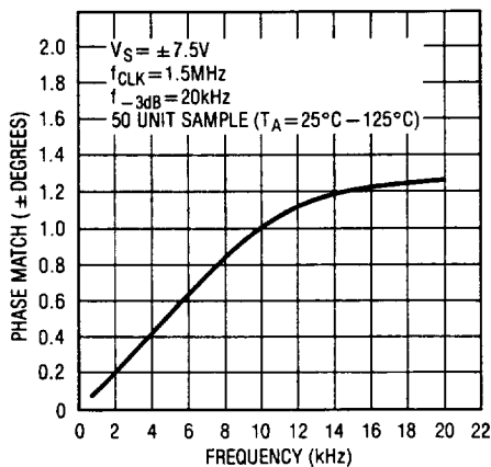
Graph 4. Phase Matching
