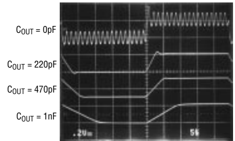
Small-Signal Response
