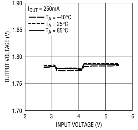
LTC1911-1.8 Output Voltage vs Input Voltage
