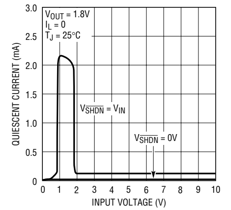
Quiescent Current
