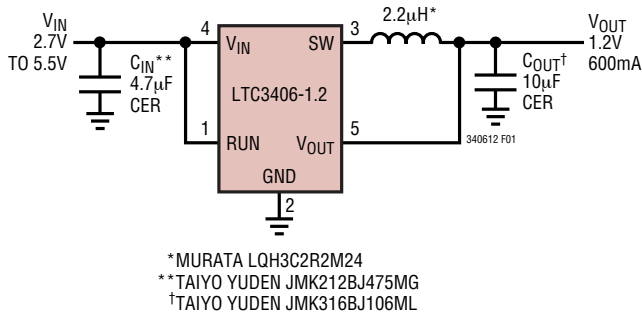
Figure 1. Typical Application
