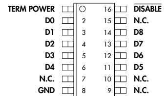
D PACKAGE (Top View)
