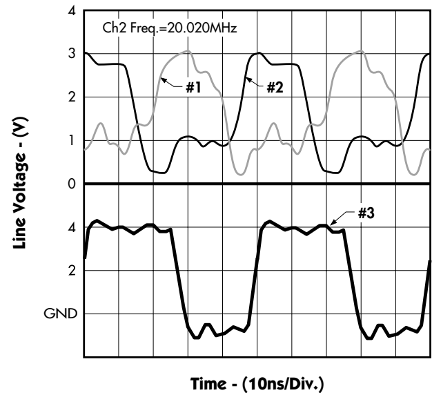
FIGURE 4. — 20MHz WAVEFORM
