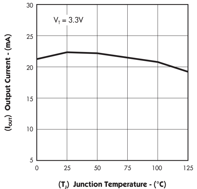
FIGURE 12. — OUTPUT CURRENT vs. JUNCTION TEMP.
