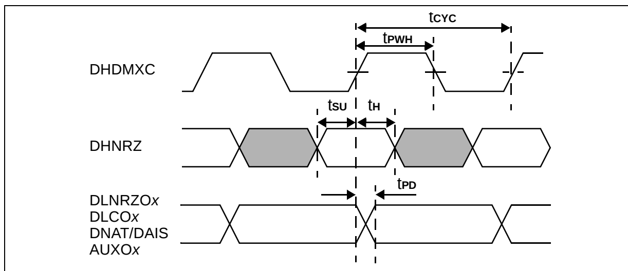
Figure 11. High Speed Demultiplexer Input &amp; Output Timing (Refer to Table 8)
