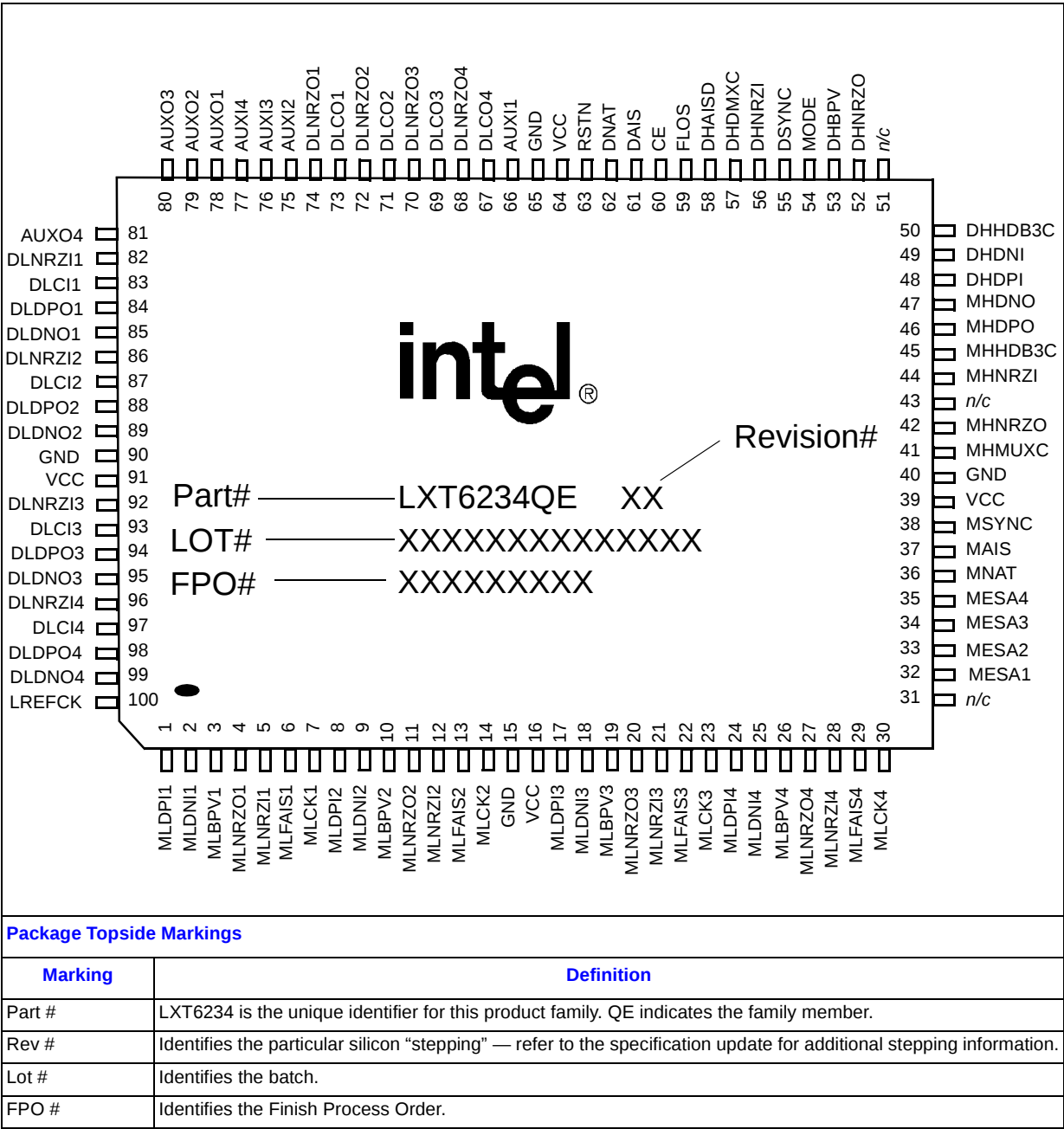
Figure 2. LXT6234 Pin Assignment
