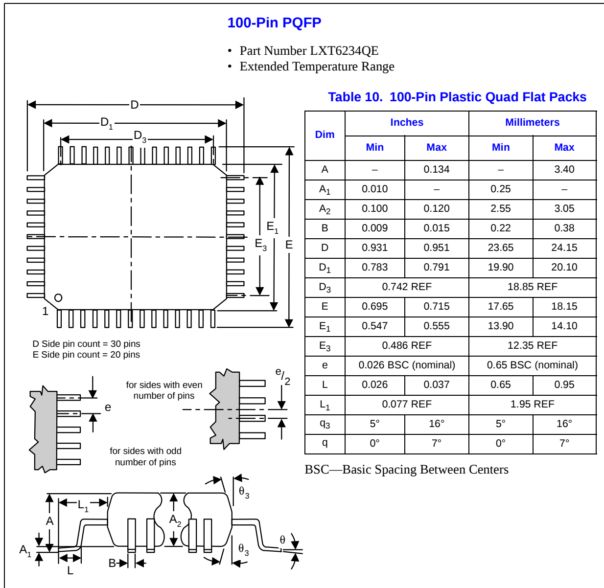
Figure 13. Package Specifications
